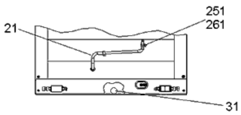
BOTTOM VIEW
