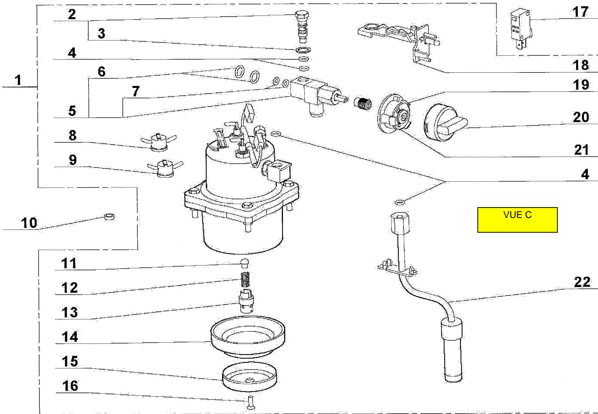
CHAUDIERE INOX - STAINLESS STEEL HEATER
