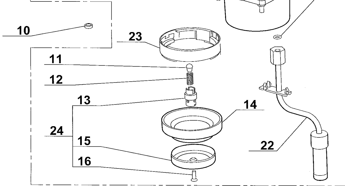
CHAUDIÈRE INOX - STAINLESS STEEL HEATER
