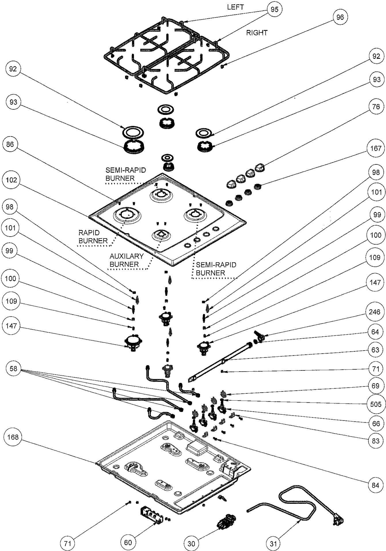
EXPLODED VIEW - 4G HOB ASSEMBLY
