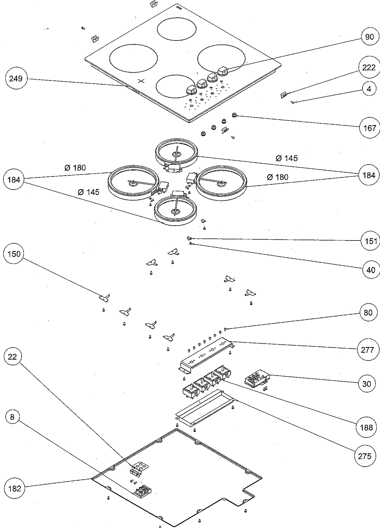
EXPLODED VIEW - RIGHT SIDE KNOB TOUCH CONTROL VITROCERAMIC HOB ASSEMBLY
