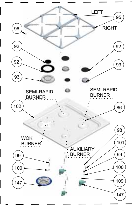
3 GAS + WOK BURNER
