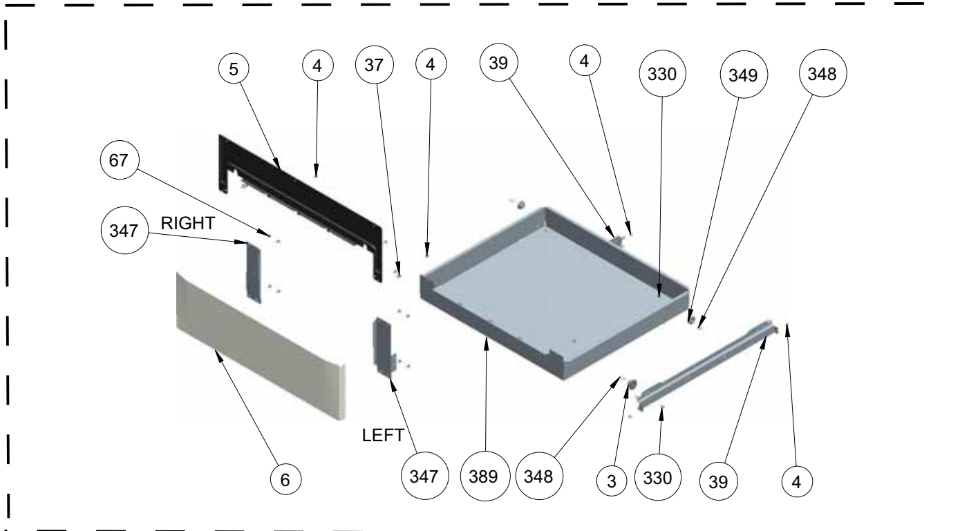
4WG DRAWER ASSEMBLY (OPTIONAL)
