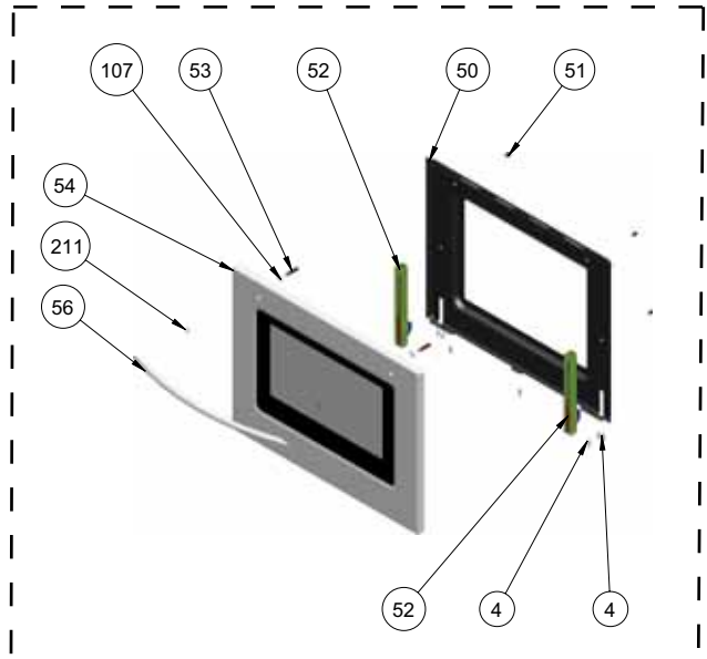
SOLID TYPE (OPTIONAL) (POSITION NO 375)
